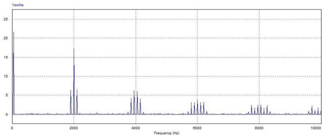
Figure 2.20: spectre de tension ( f_p=2 kHz, V_m= 4.5V ).
