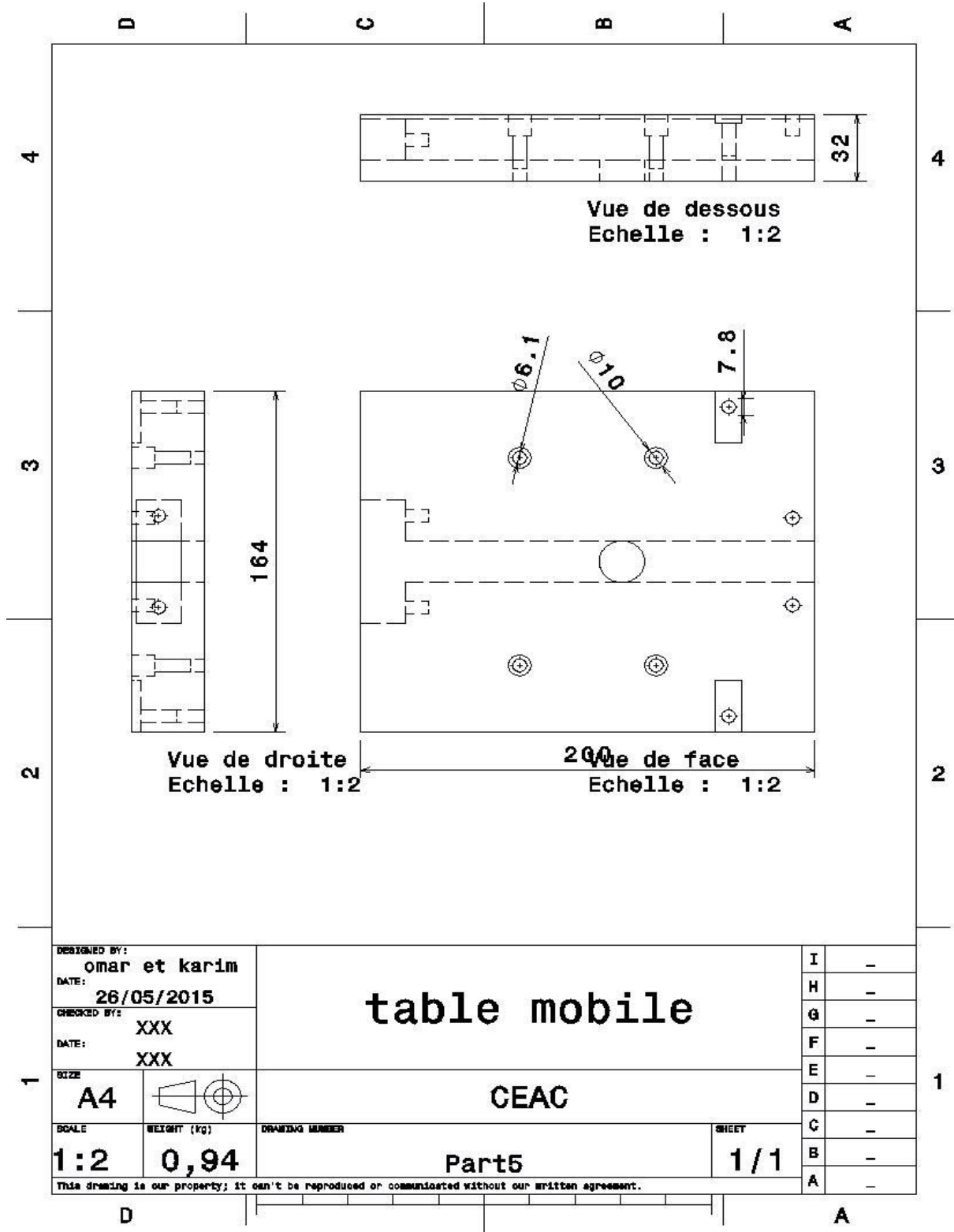
Figure 49: Drafting de table mobile .
