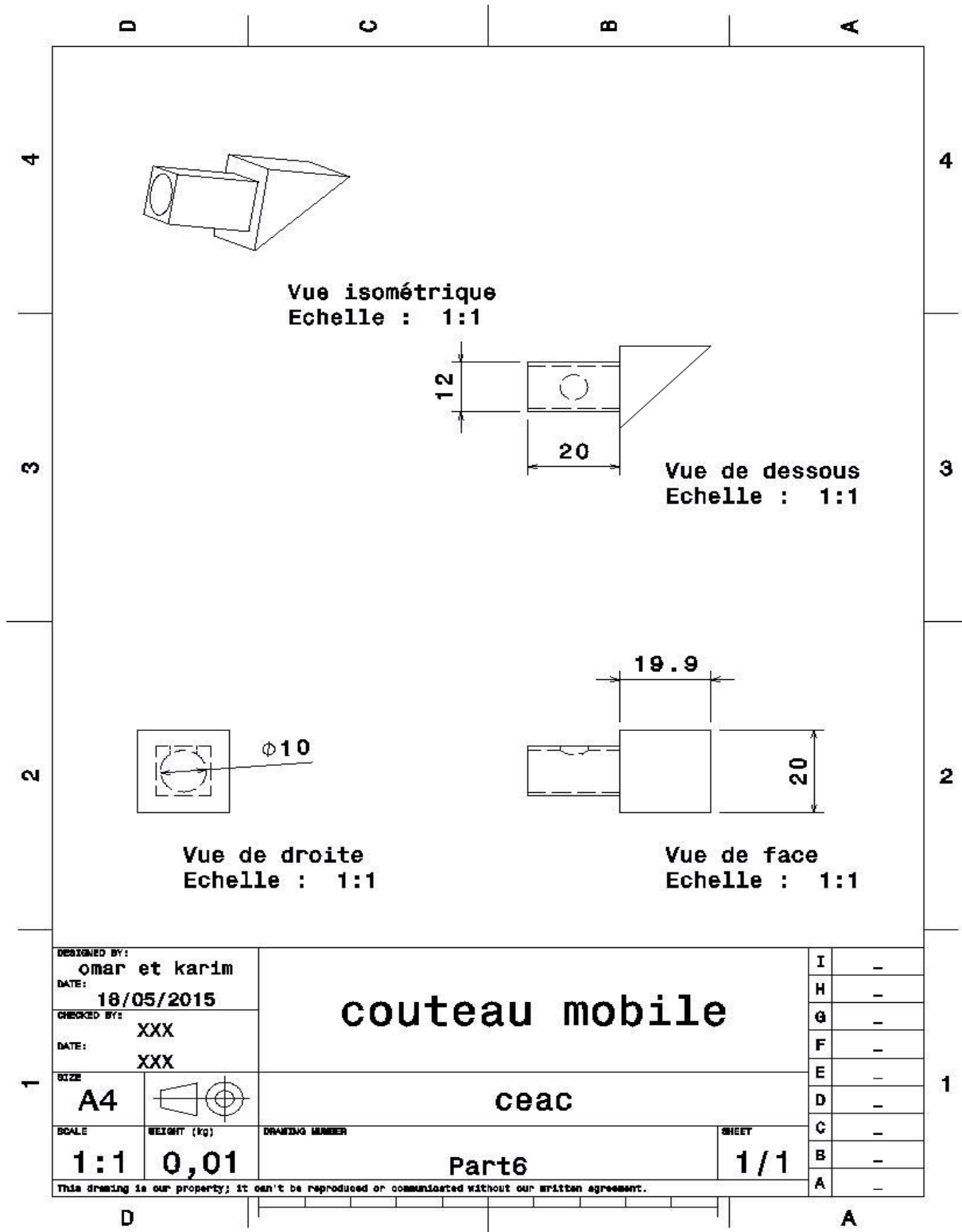
Figure 44: Drafting de couteau mobile.
