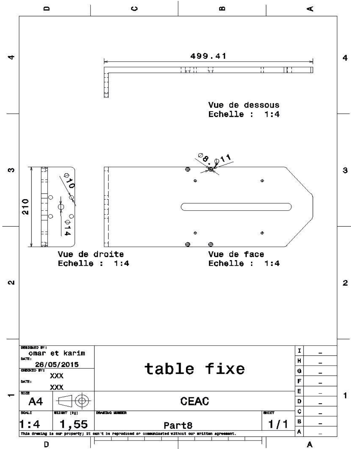
Figure 48: Drafting de table fixe.
