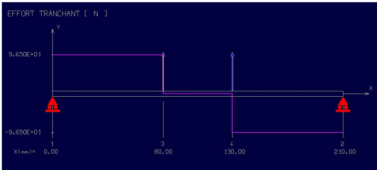
Figure 20: Diagramme des efforts tranchants.
