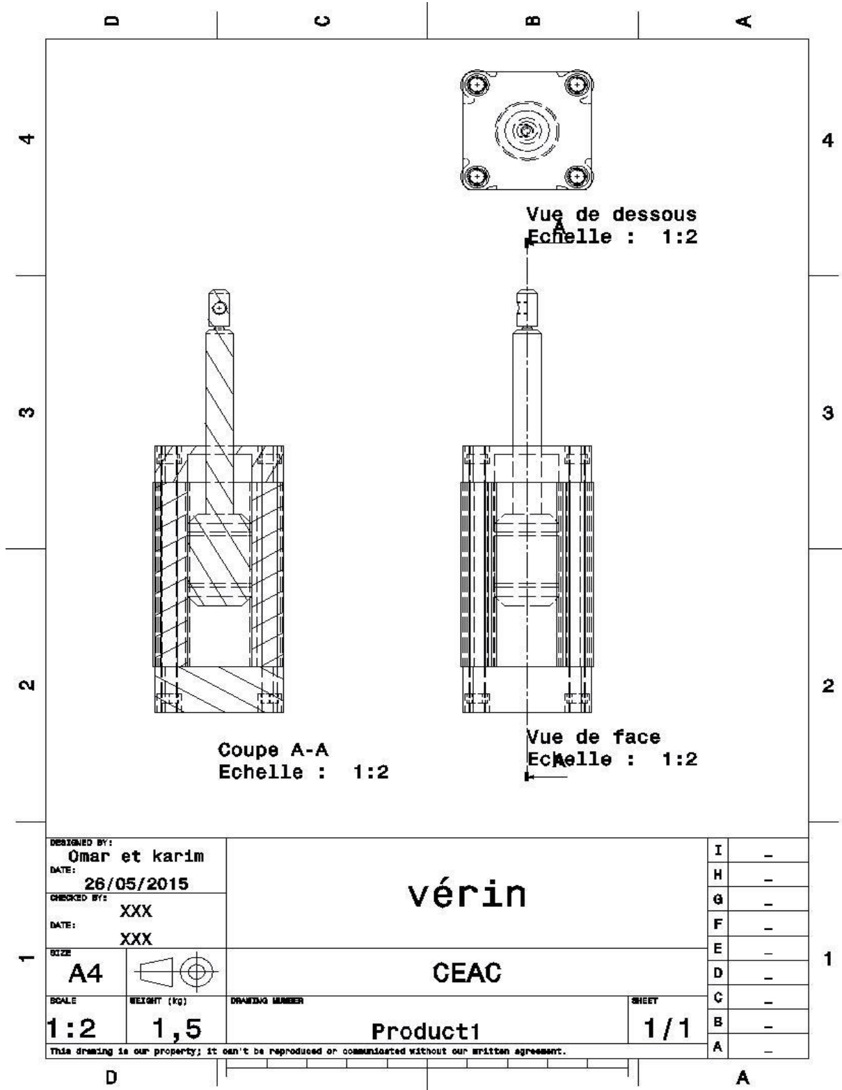
Figure 51: Drafting de vérin.
