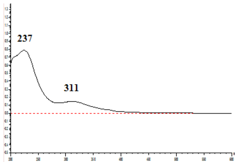
Figure 8 : Spectre des bandes UV-visible de H_4PMo_{11}VO_{40}
