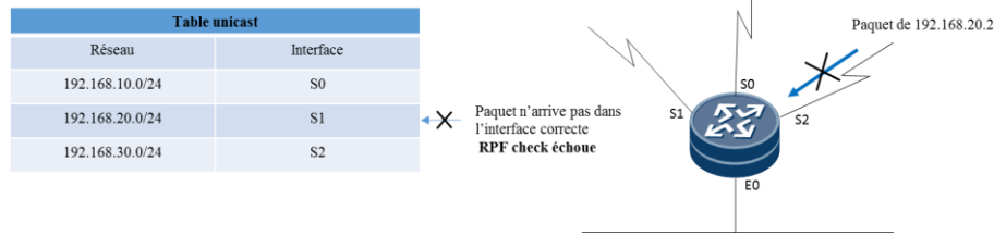
Figure 25: RPF check échoue. [4]
