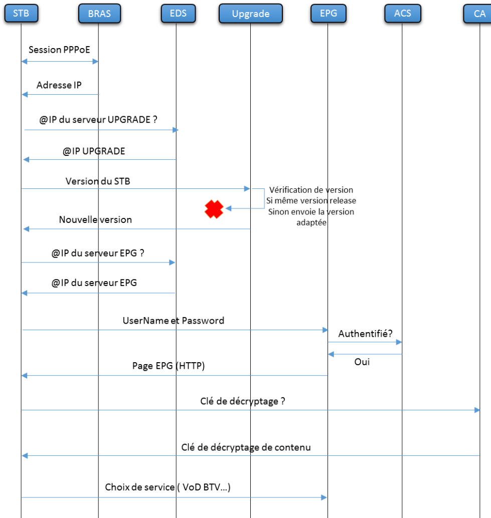
Figure 19: Initialisation STB.
