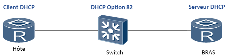
Figure 65: Relais DHCP Option 82.
