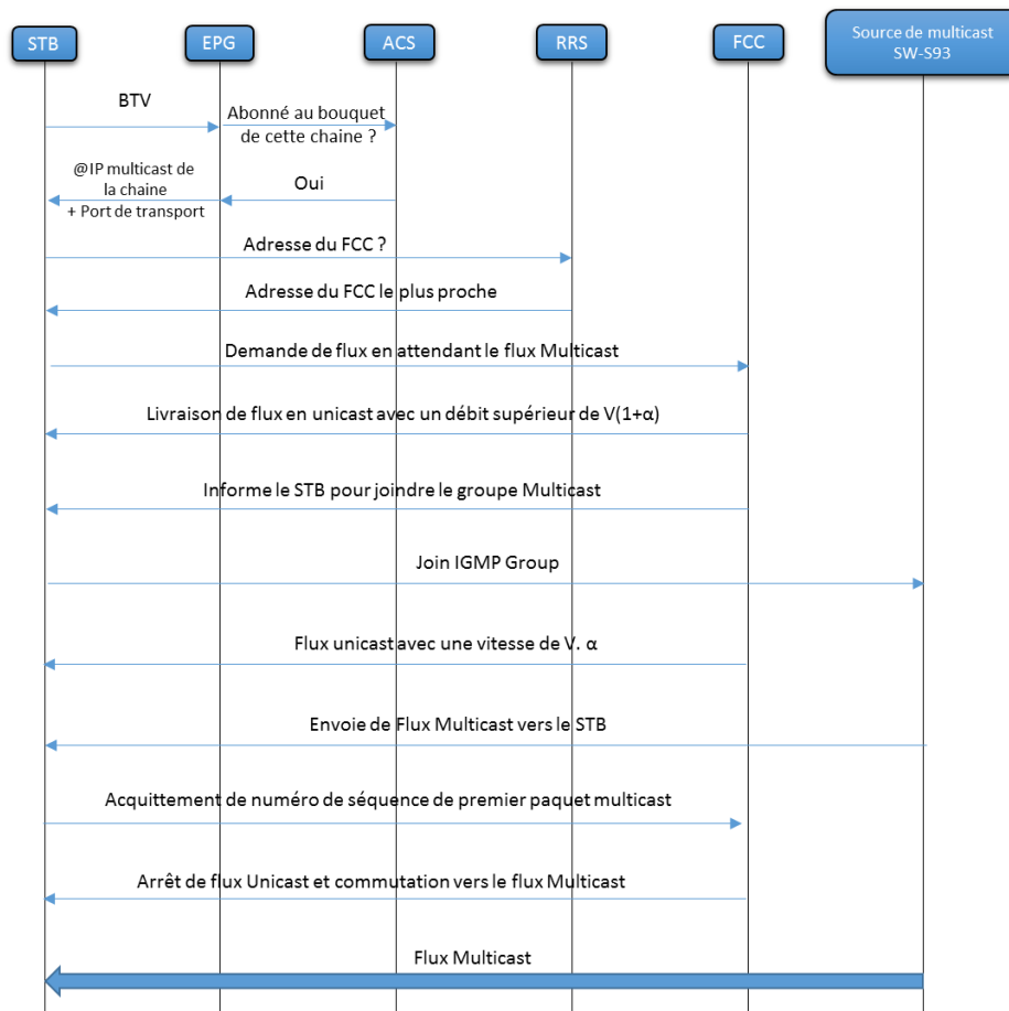
Figure 21: Service BTV.
