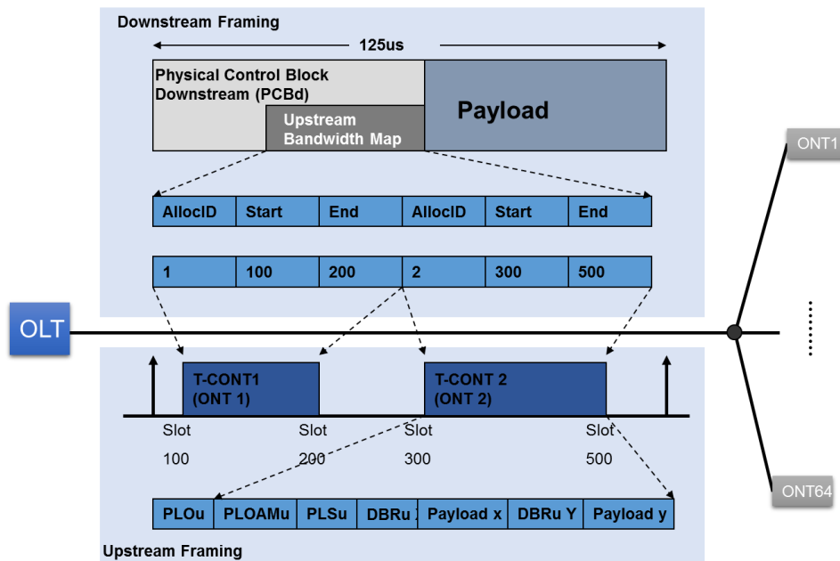
Figure 98: Structure de la trame GPON. [18]
