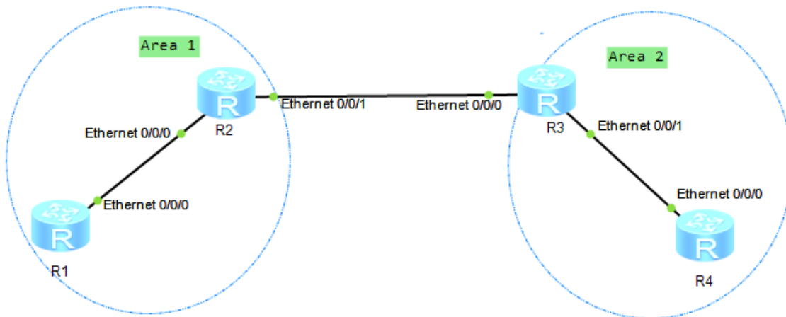
Figure 69: Simulation du protocole IS-IS.
