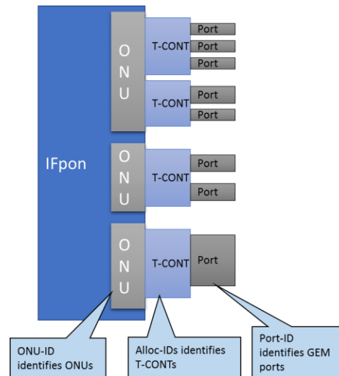
Figure 97: Architecture de multiplexage en GPON. [18]
