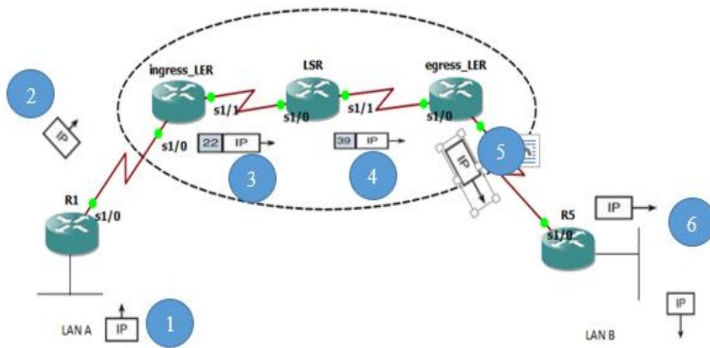
Figure 79: Simulation du MPLS.
