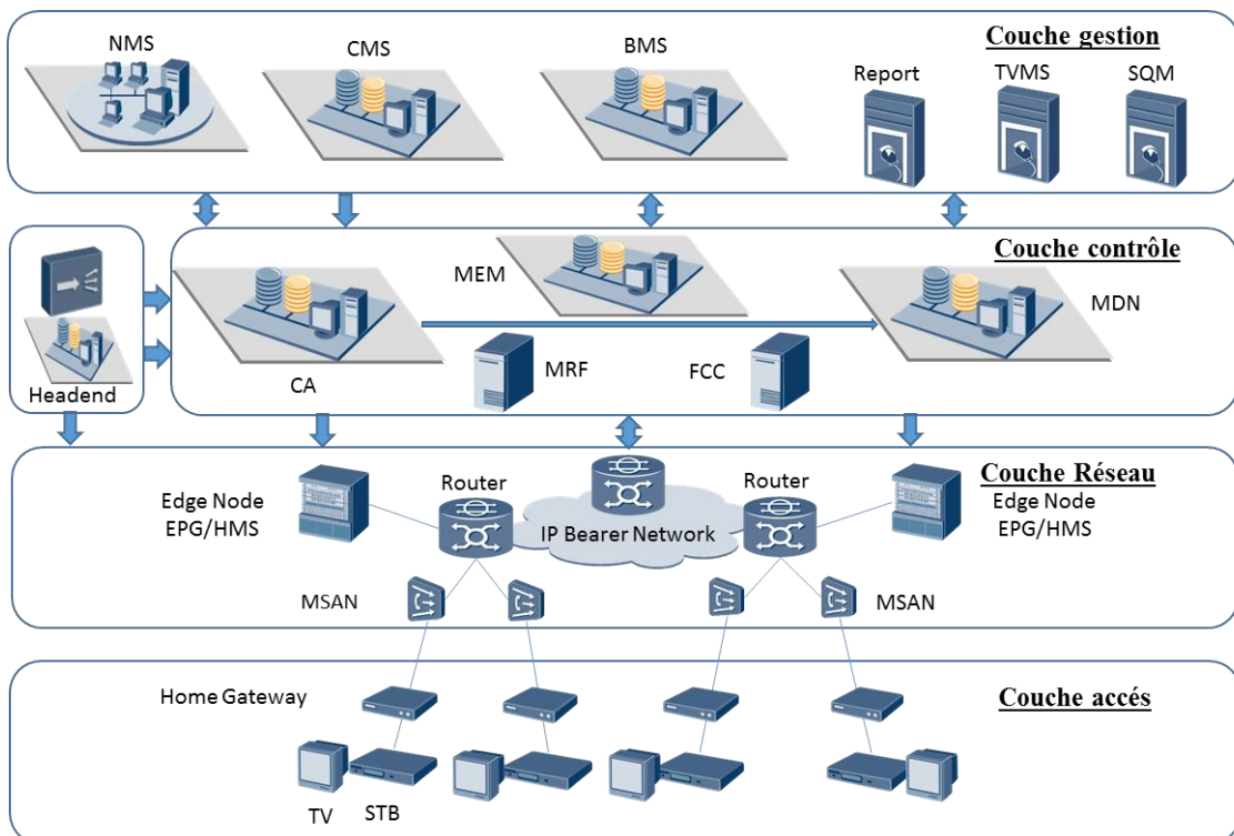
Figure 10: Architecture de la plateforme IPTV. [1]
