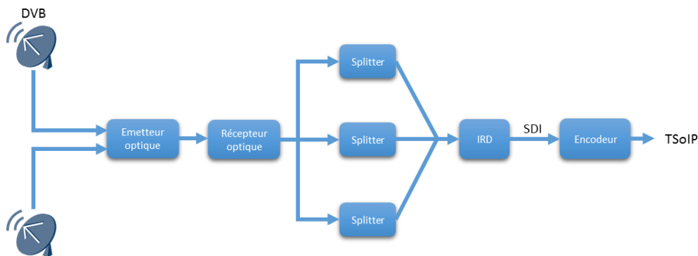
Figure 11: Composants du HeadEnd. [1]
