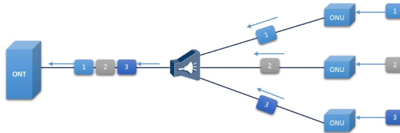
Figure 96: Transmission en upstream en TDMA. [18]
