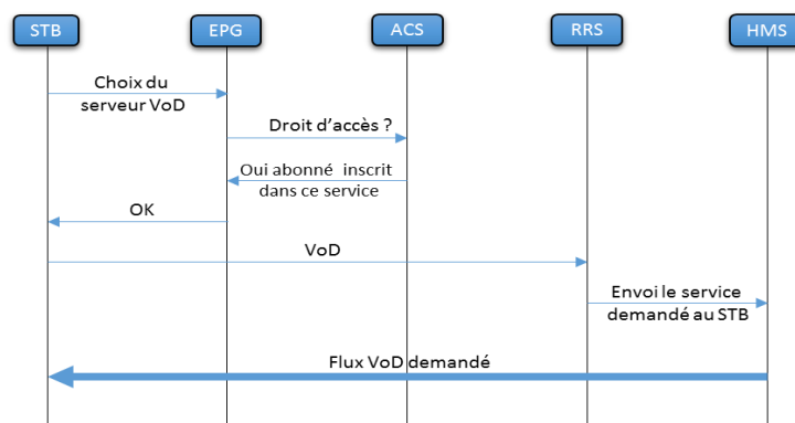
Figure 20: Service VoD.
