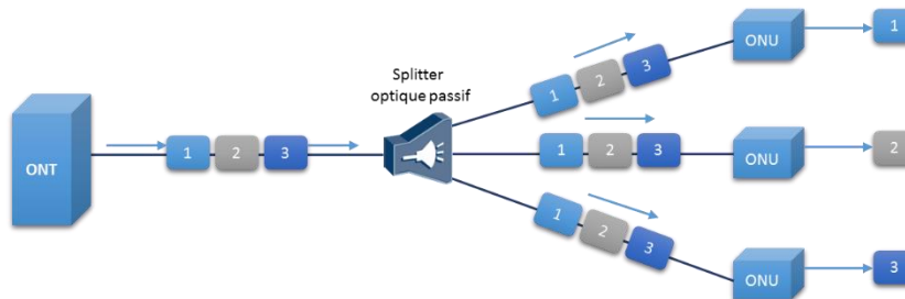
Figure 95: Transmission des services. [18]
