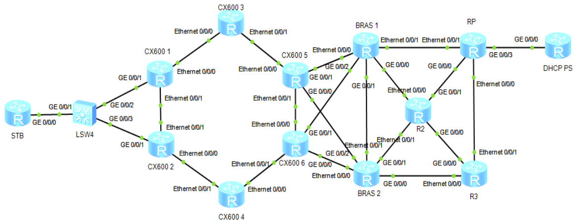
Figure 51: Simulation du protocole DHCP.
