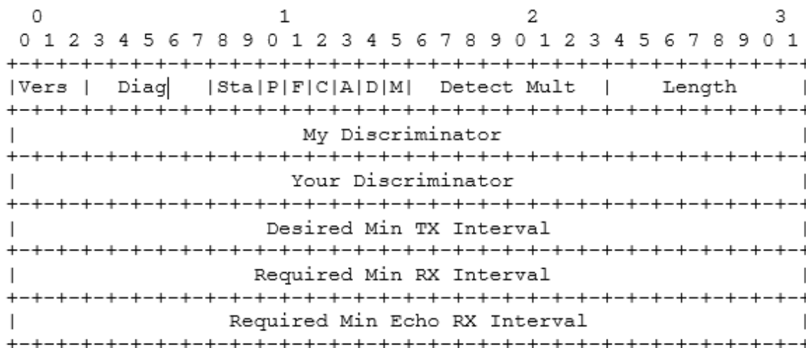
Figure 85: Format du paquet BFD. [17]
