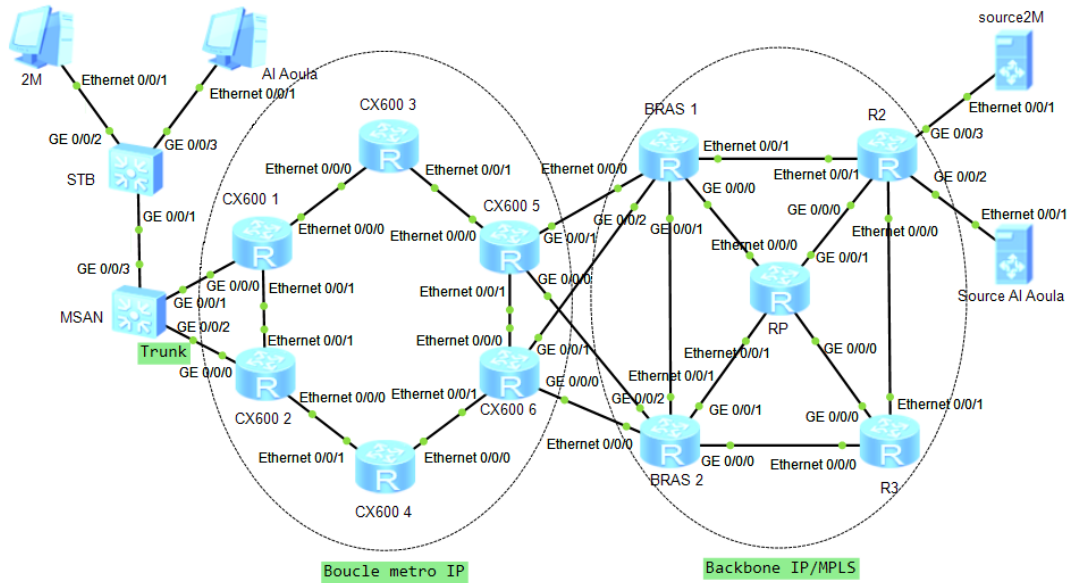
Figure 38: Simulation end-to-end de la solution IPTV.
