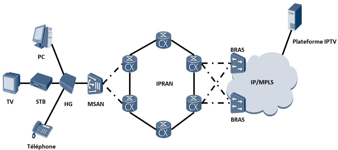
Figure 22: Architecture end-to-end de la solution IPTV.
