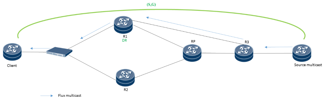
Figure 27: Switch Over.
