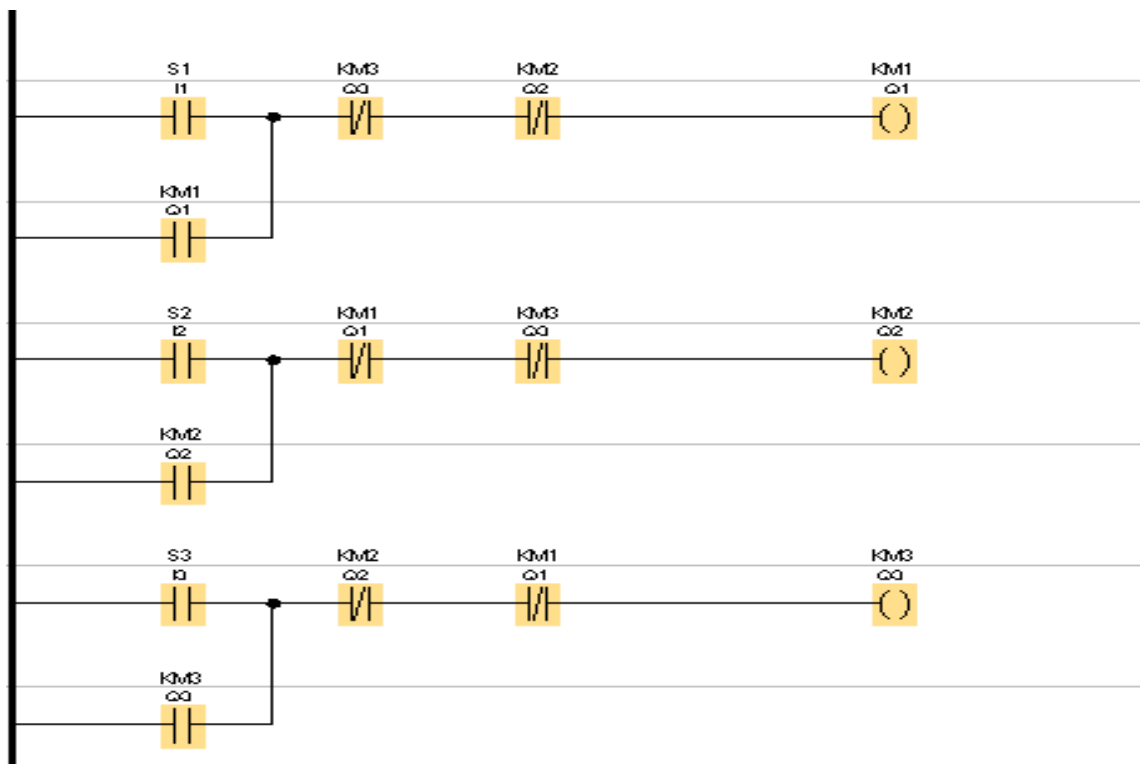
Figure 15 : Programme LADDER
