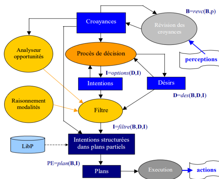
Figure 7: Architecture BDI [34]
